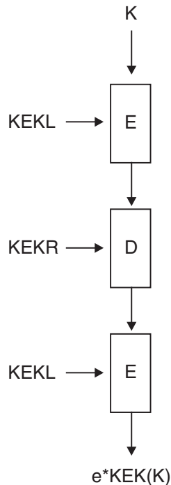
Figure 21. Multiple Encipherment of Single-length Keys
