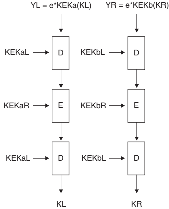
Figure 24. Multiple Decipherment of Double-length Keys
