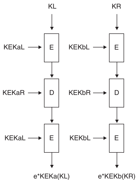
Figure 23. Multiple Encipherment of Double-length Keys
