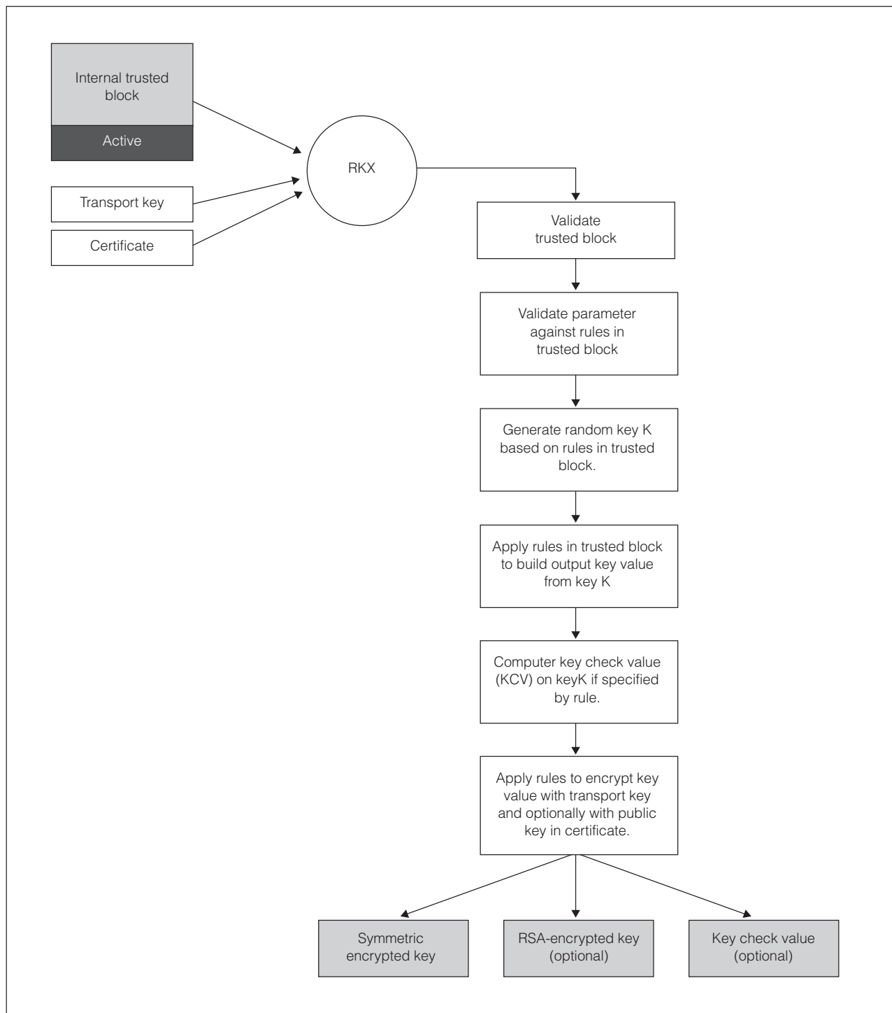
Figure 6. Generating keys using a trusted block
