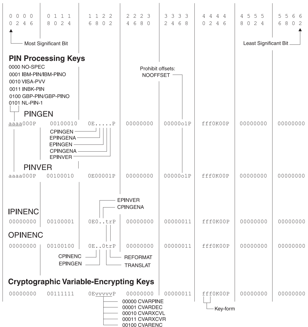
Figure 11. Control Vector Base Bit Map (PIN Processing Keys and Cryptographic Variable-Encrypting Keys)
