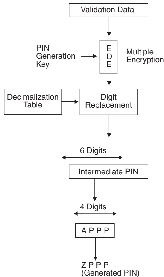
Figure 16. GBP PIN Generation Algorithm
