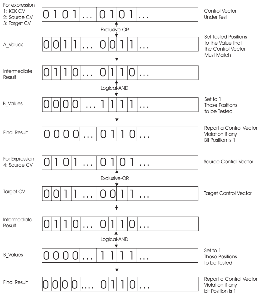
Figure 13. Control Vector Translate Callable Service Mask_Array Processing
