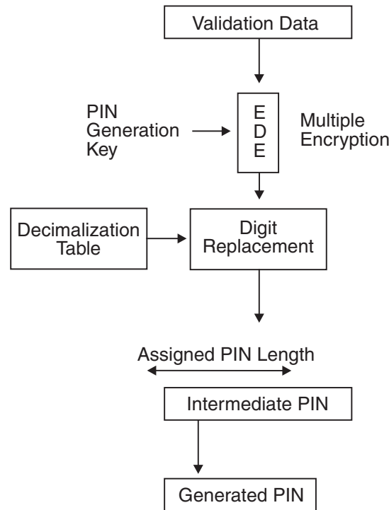
Figure 15. 3624 PIN Generation Algorithm
