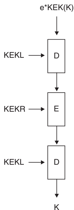
Figure 22. Multiple Decipherment of Single-length Keys
