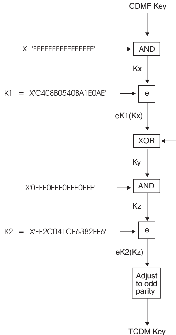
Figure 27. The CDMF Key Transformation Algorithm
