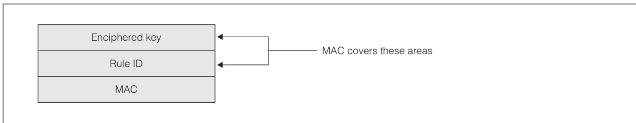
Figure 3. Simplified RKX key-token structure
