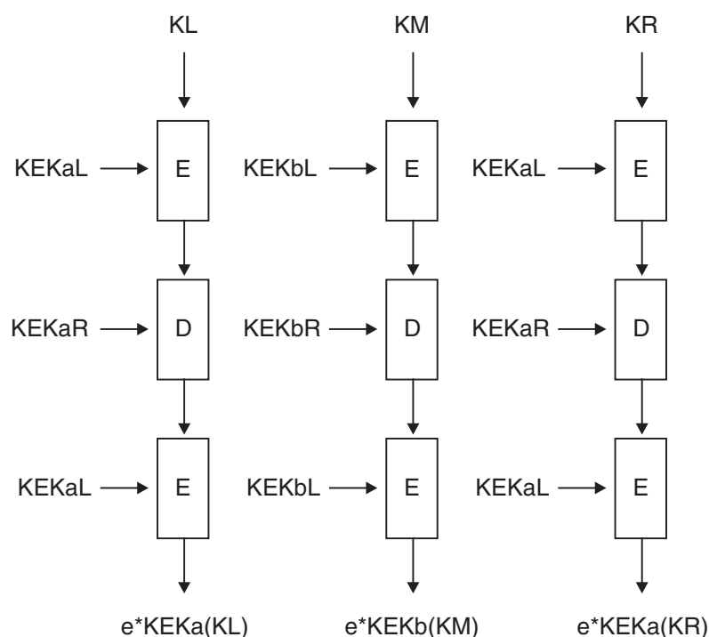
Figure 26. Multiple Decipherment of Triple-length Keys
