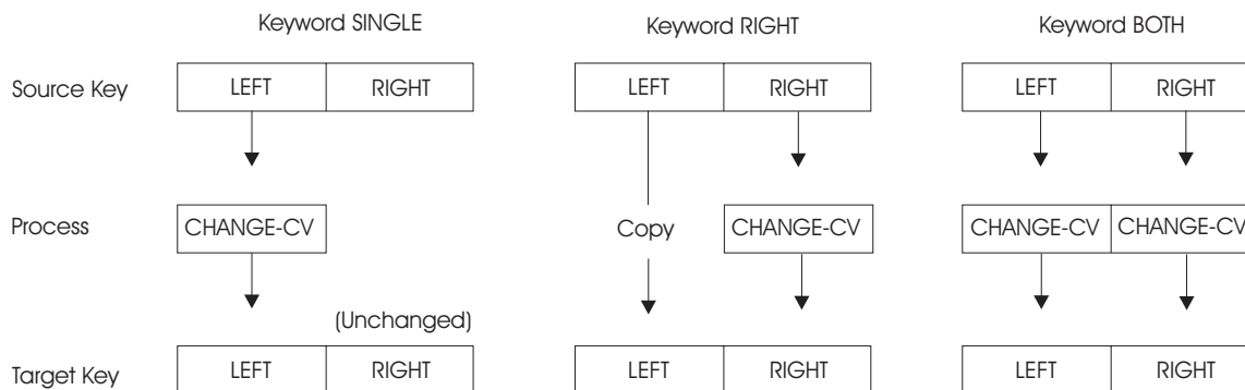
Figure 14. Control Vector Translate Callable Service. In this figure, CHANGE-CV means the requested control vector translation change; LEFT and RIGHT mean the left and right halves of a key and its control vector.
