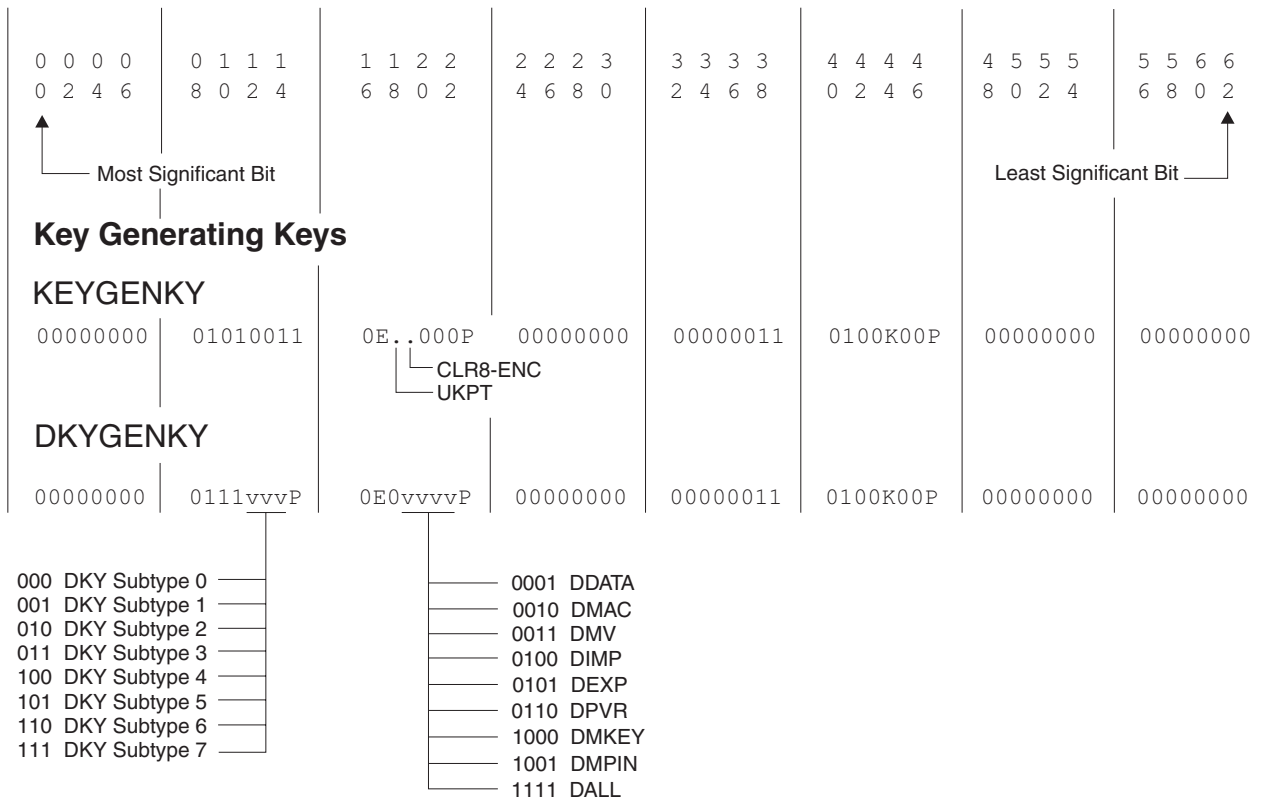
Figure 12. Control Vector Base Bit Map (Key Generating Keys)
