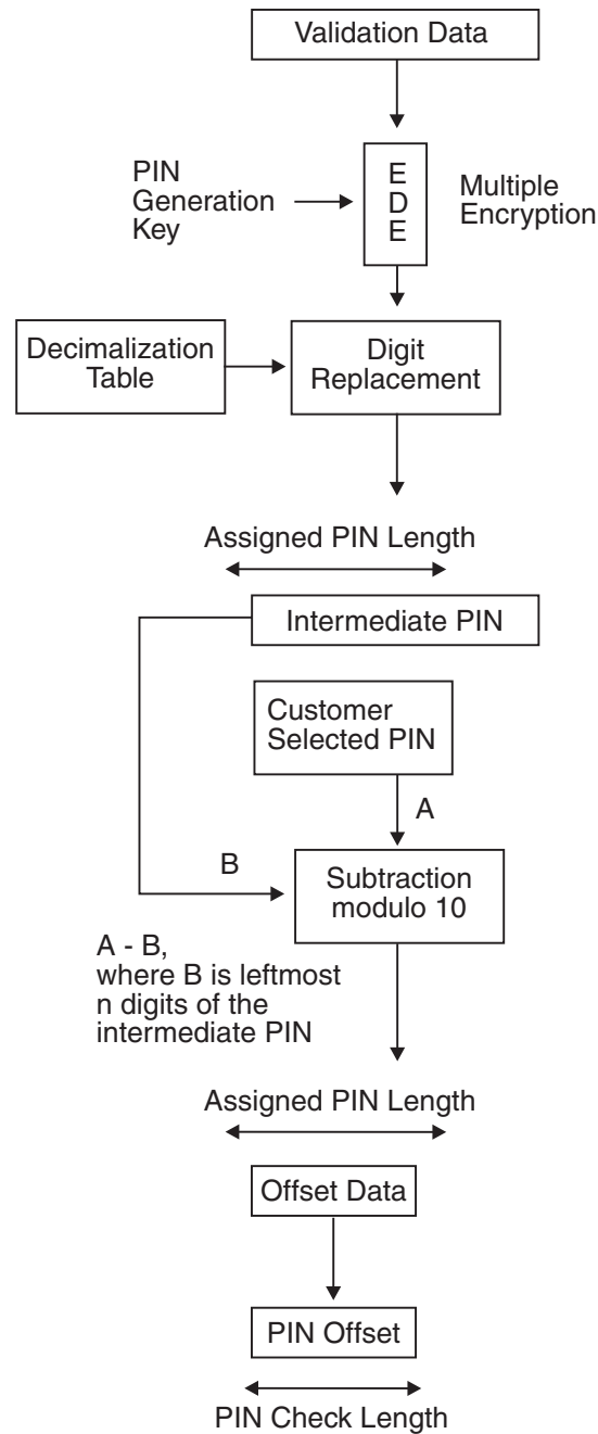
Figure 17. PIN-Offset Generation Algorithm
