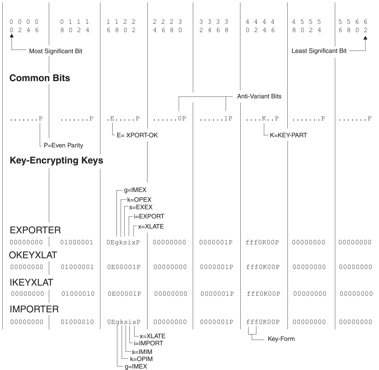
Figure 9. Control Vector Base Bit Map (Common Bits and Key-Encrypting Keys)
