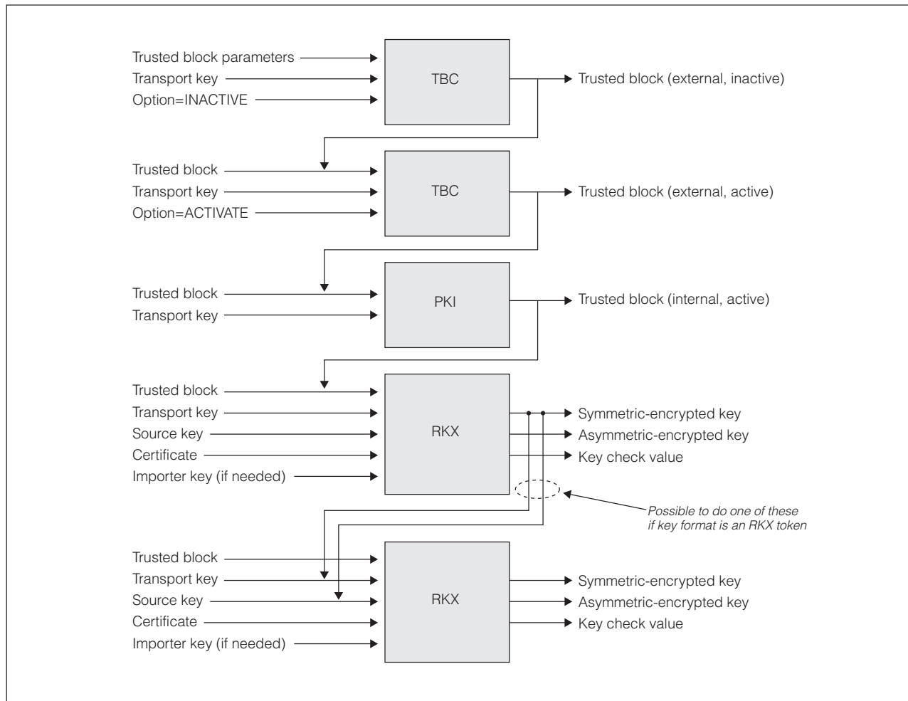
Figure 7. Typical flow of verbs for remote key export
