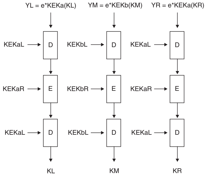
Figure 25. Multiple Encipherment of Triple-length Keys
