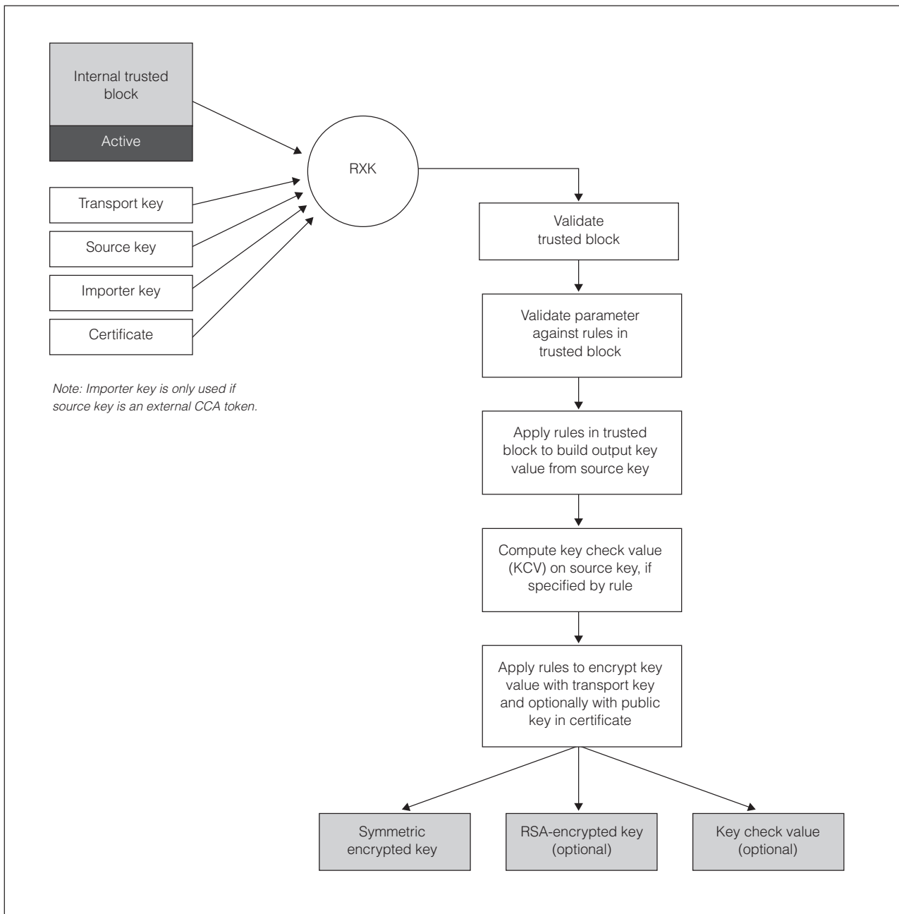
Figure 5. Exporting keys using a trusted block
